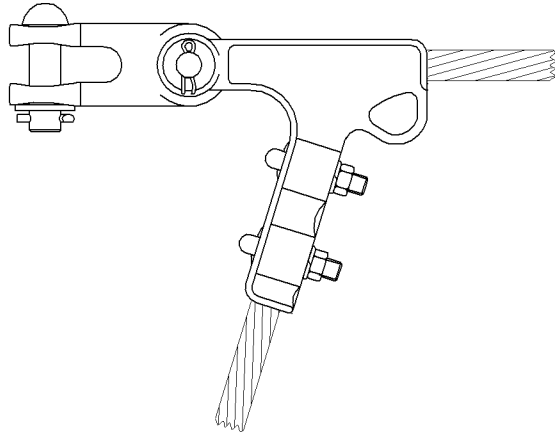
Single Strain Earth Wire Assembly
