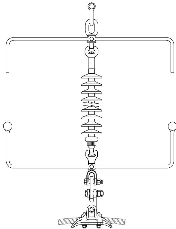
Single Suspension Twin Conductor Assembly
