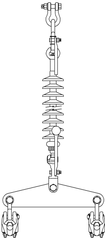
Single Suspension Twin Conductor Assembly
