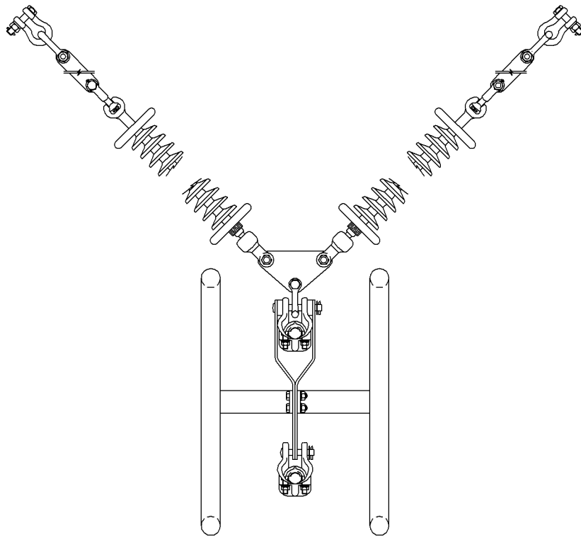
”V” Suspension Twin Conductor Assembly
