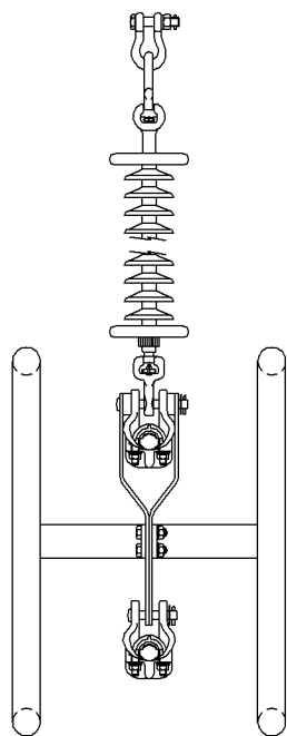
Single Suspension Twin Conductor Assembly
