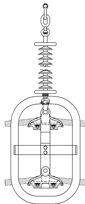
Single Suspension Twin Conductor Assembly
